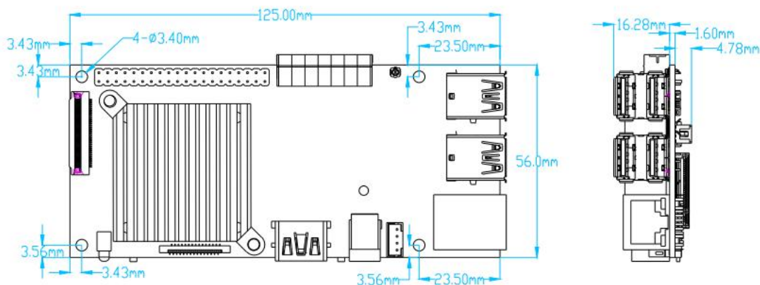
Figure 4 Product illustration dimensions
