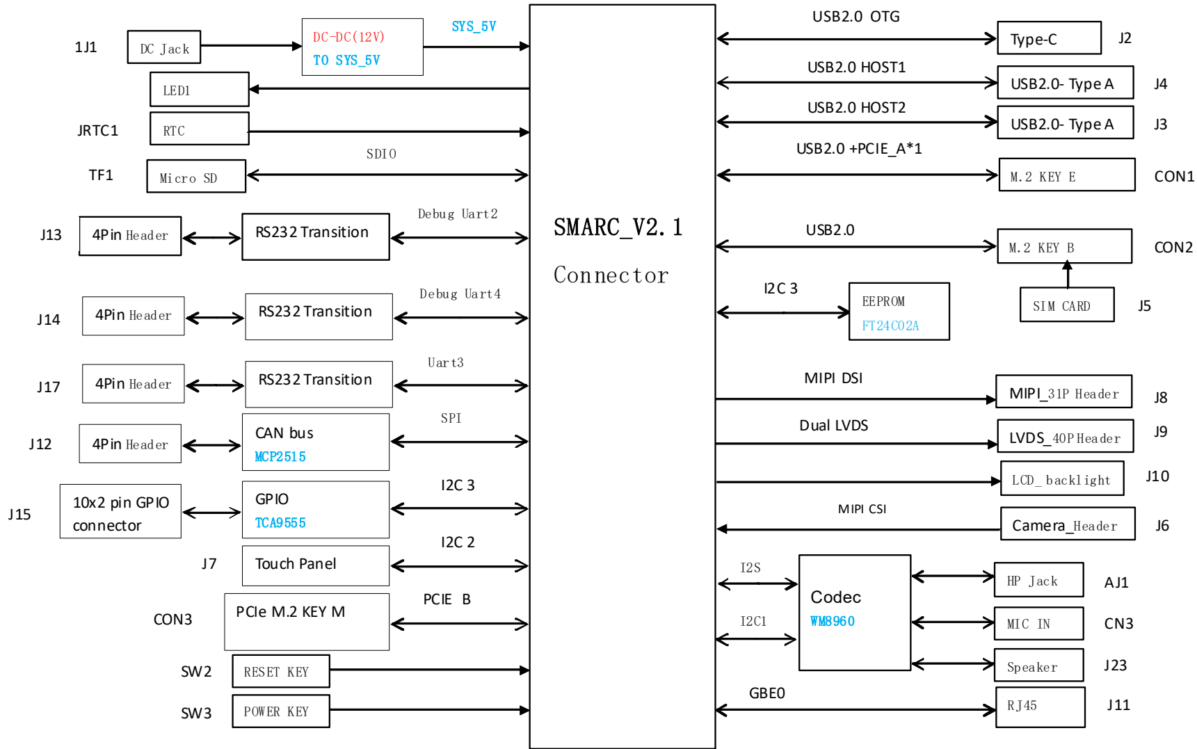
SMA_Baseboard_Block diagram (VER:A02)
