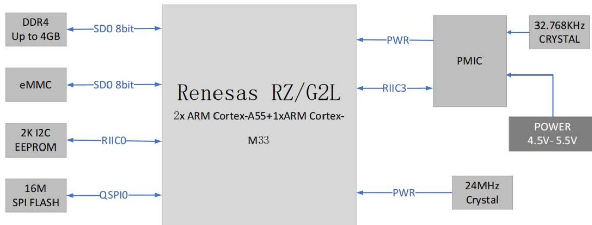
Figure 2 Core board hardware block diagram
