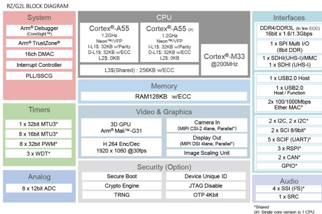
Figure 3 RZ/G2L processor architecture diagram
